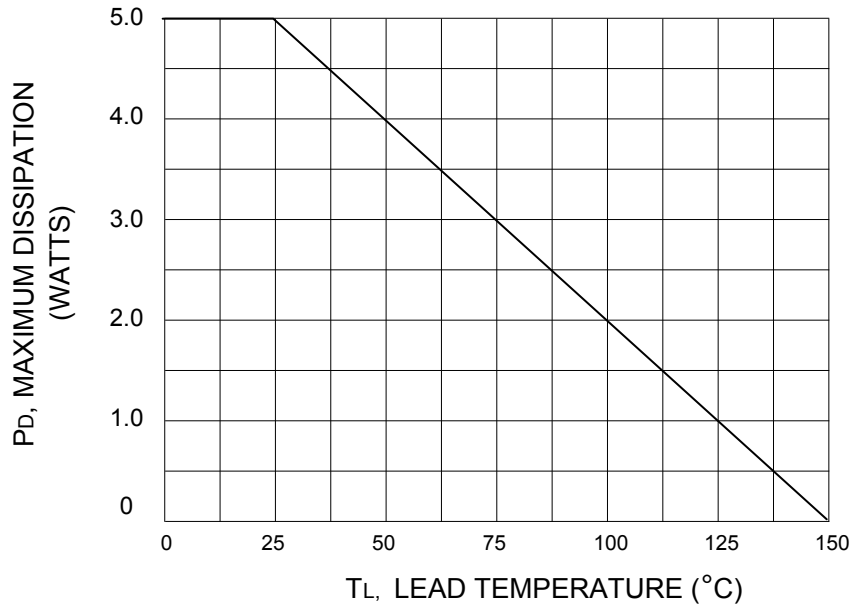
Fig. 1 POWER DERATING CURVE
